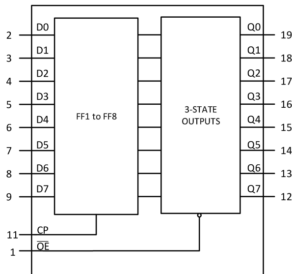
Fig. 1. Functional diagram
